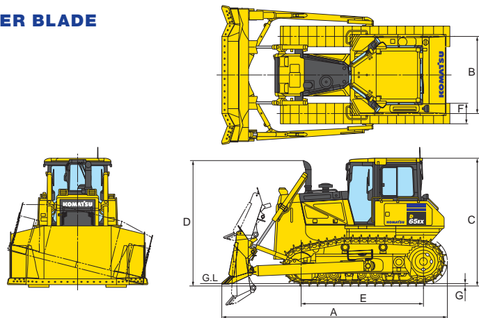
Shown with SIGMADOZER® (D65EX-18) single grouser shoe.
